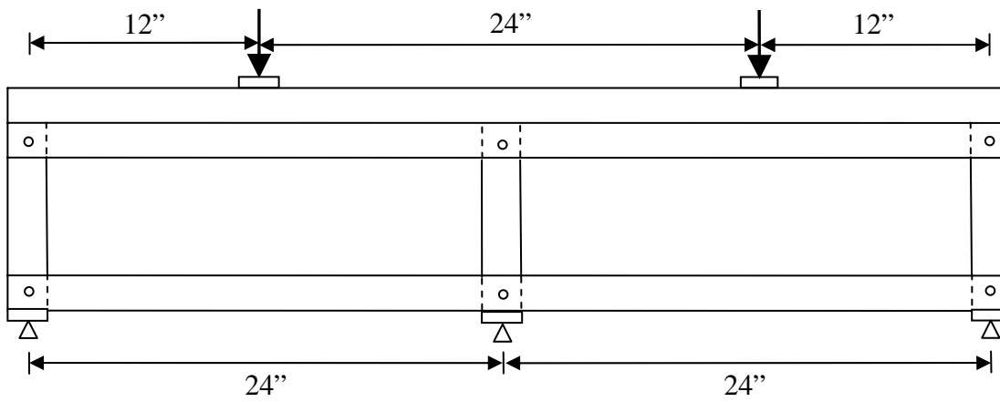
Figure 3.2 – Typical Test Setup of 24 Inch Specimen
