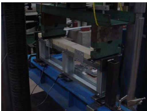
Figure 4.3 –Specimen 2A16-18 with shear plates
