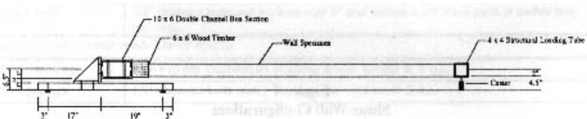
FIGURE 3 Elevation of Shear Wall Testing Layout
