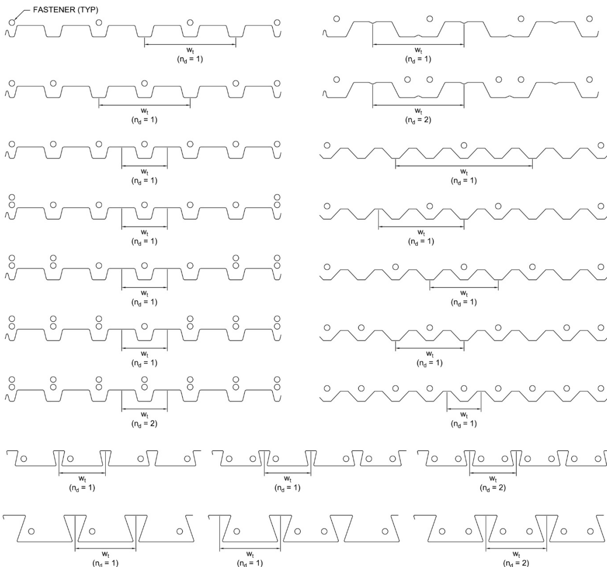
Figure C-D1-1 Tributary Width and Number of Fasteners for Various Attachment Patterns
