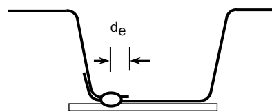
Figure C-D1-3 Nestable Sidelap
