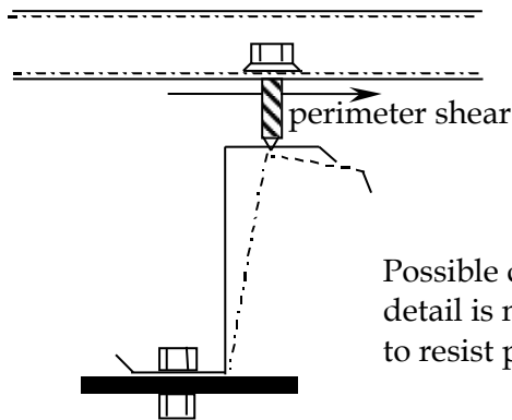
Figure C-D5.1.1-1 Example of Purlin Roll
