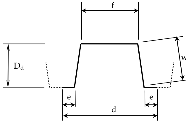
Figure 1.4-1 Panel Configuration
