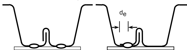
Figure C-D1-2 Interlocking Sidelaps
